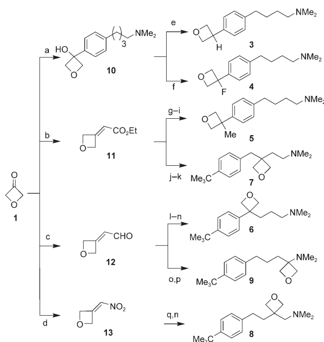
Scheme 1. a) (Me 2 N)(CH 2 ) 4 (C 6 H 4 )- p -Li, THF, −78 °C, 71%; b) Ph 3 PCHCO 2 Et, CH 2 Cl 2 , RT, 89%; c) Ph 3 PCHCHO, CH 2 Cl 2 , RT, 81%; d) 1. NEt 3 , MeNO 2 , RT; 2. NEt 3 , MsCl, CH 2 Cl 2 , −78 °C, 81%; e) 1. NaH, Et 2 O, 0 °C; 2. TsCl, 0 °C; 3. LiAlH 4 , −78 °C, 58%; f) DAST, CH 2 Cl 2 , −78 °C, 40%; g) (Me 2 N)(CH 2 ) 4 (C 6 H 4 )- p -B(OH) 2 , cat. [(Rh-(cod)Cl) 2 ], KOH, aq dioxane, RT, 83%; h) DIBAL-H, −78 °C; i) [(Ph 3 P) 3 RhCl], toluene, 105 °C, 33% (2 steps); j) 4- t -BuBnMgBr, TMSCl, CuI, THF, −18 °C, 70%; k) Me 2 NH, NaCNBH 3 , MeOH, 28% (2 steps); l) 4- t -BuPhB(OH) 2 , cat. [(Rh-(cod)Cl) 2 ], KOH, aq dioxane, RT, 78%; m) 1. MeNO 2 , NEt 3 , RT; 2. NEt 3 , MsCl, CH 2 Cl 2 , −78 °C, 58%; n) 1. H 2 , Pd(OH) 2 /C, CH 2 O, RT, MeOH; 2. NaCNBH 3 , CH 2 O, MeOH, 34% o) 1. HNMe 2 , DBU, THF, −18 °C; 2. 4- t -BuPhCHPh 3 ; p) H 2 , Pd/C, MeOH, 36% (3 steps); q) (E)-4- t -BuC 6 H 4 CHCH(OH) 2 , cat. [(Rh-(cod)Cl) 2 ], KOH, aq dioxane, RT; 34% (overall sequence). Ms = methanesulfonyl, Ts = toluene- p -sulfonyl, DAST = (diethylamino)sulfur trifluoride, cod = cycloocta-1,5-diene, DIBAL-H = diisobutylaluminum hydride, TMS = trimethylsilyl, DBU = 1,8-diazabicyclo[5.4.0]undec-7-ene, Bn = benzyl.
