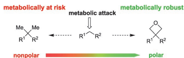
Figure 1. Comparison of gem -dimethyl and oxetane modules.
